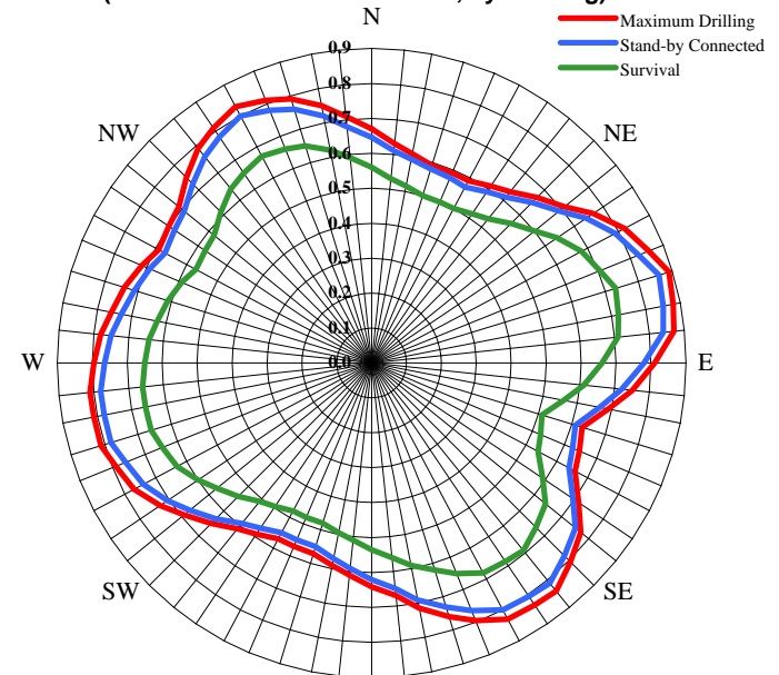
T+12 Forecast Roll (10 minute max values at COG, by heading)
