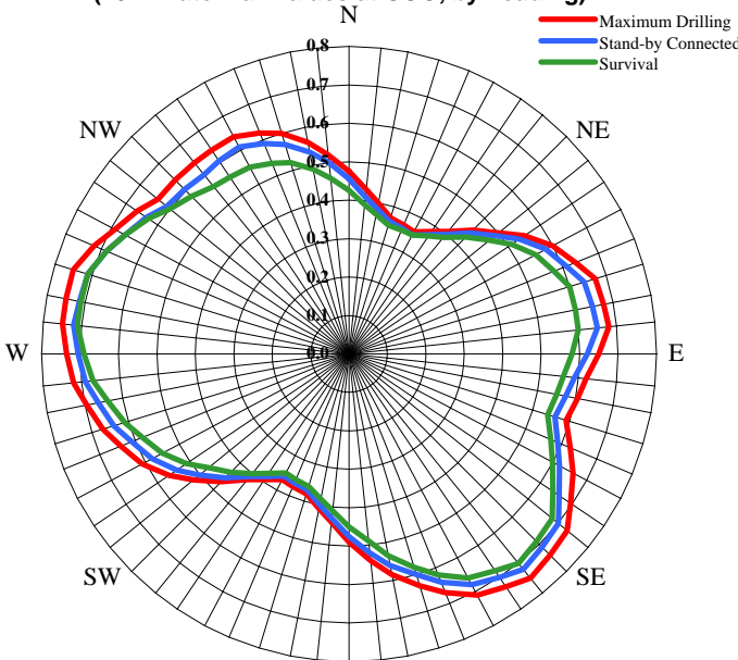
T+6 Forecast Roll (10 minute max values at COG, by heading)
