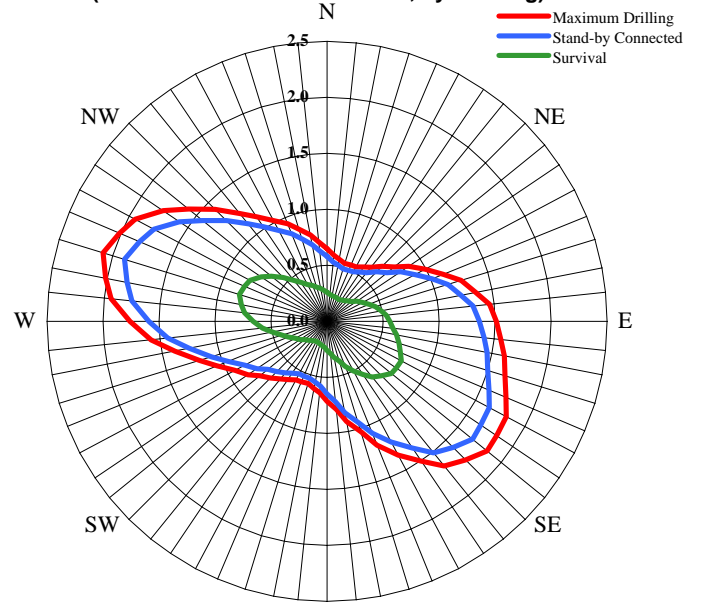
T+12 Forecast Pitch (10 minute max values at COG, by heading)
